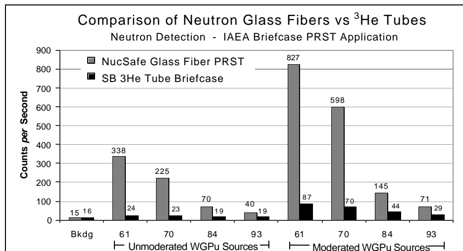
Figure 3. Comparisons of data collected with a glass fiber neutron sensor with those from 5 ^3\text{He} tubes at 3 atmospheres measuring 25 cm in length by 2.5 cm in diameter.
