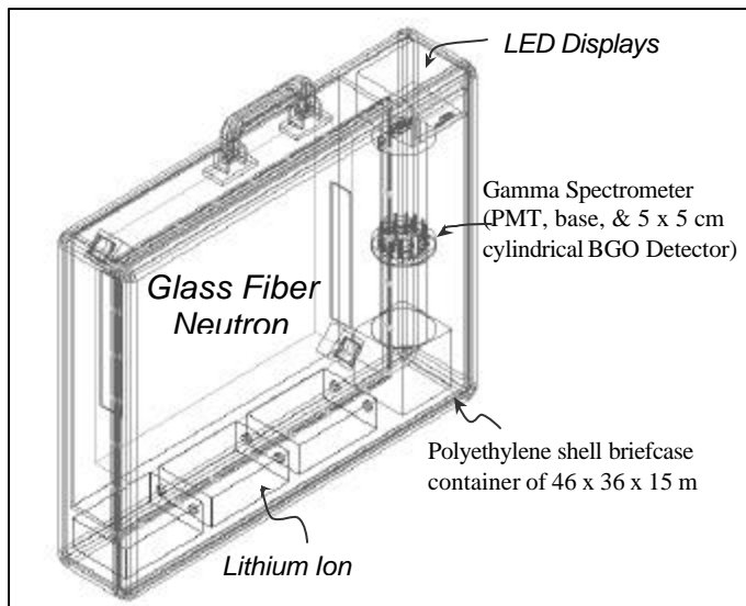
Figure 1. Modified 3D CAD drawing of the NucSafe PRST. The system has been designed to be as modular as possible. Neutron and gamma ray sensors are removable and easy to replace with alternate sensor / detection sub-systems.
