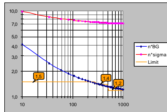
Fig. 2: Minimum nominal threshold setting as function of multiples of Background and sigma.
