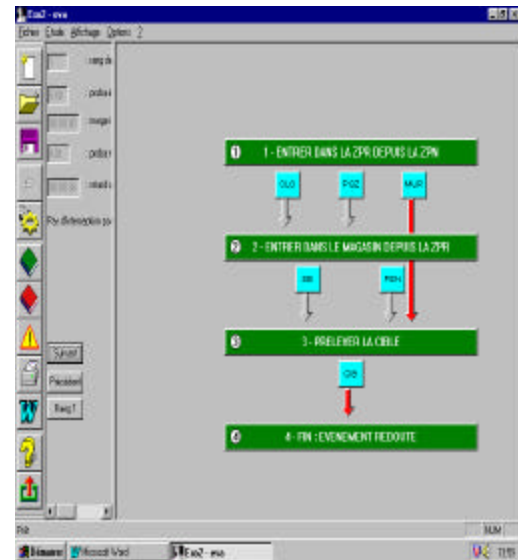
fig. 2 : EVA Software : Diagram of a hypothetical facility with various ways to reach the target, probability of detecting intruders, probability of intercepting intruders, margin or the delay of the intervention force, critical detection point, most vulnerable passage areas.
