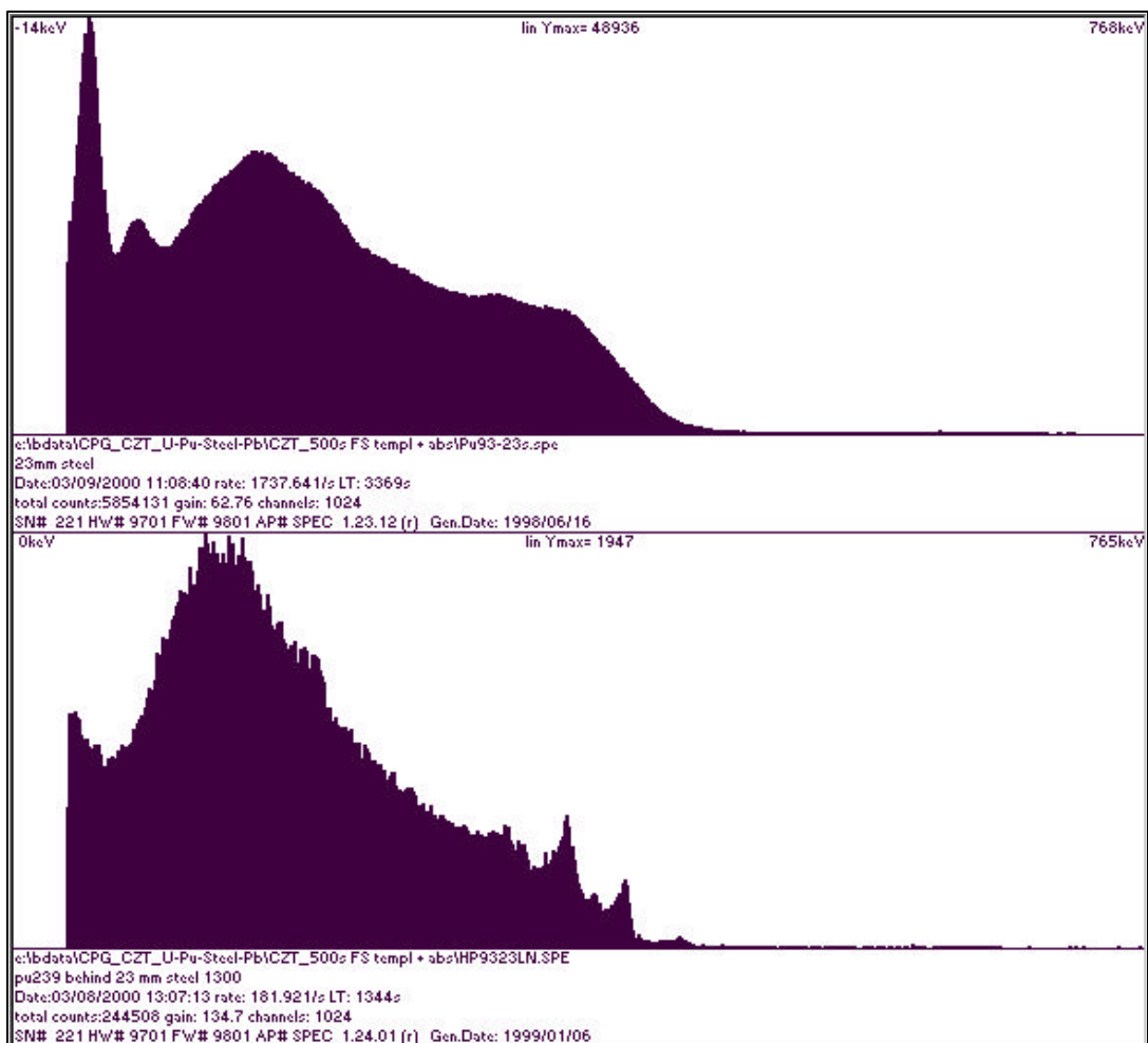
Figure 1 Comparison of gamma spectra of a Pu source (93% Pu-239; 23mm steel shielding) measured with NaI detector (upper trace) and with CZT/500 detector (lower trace). Only the spectrum taken with the CZT/500 detector shows enough gamma peak information which allows to identify Pu.
